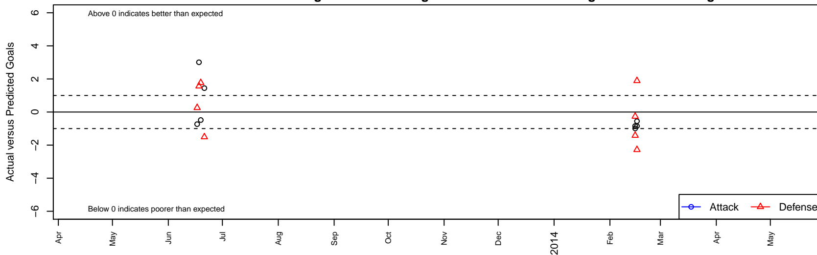
Colorado Storm 00 Copa B99 Dots are actual minus expected GF (blue circles) and GA (red triangles). Blue line is smoothed change in attack strength. Red is smoothed change in defense strength.
